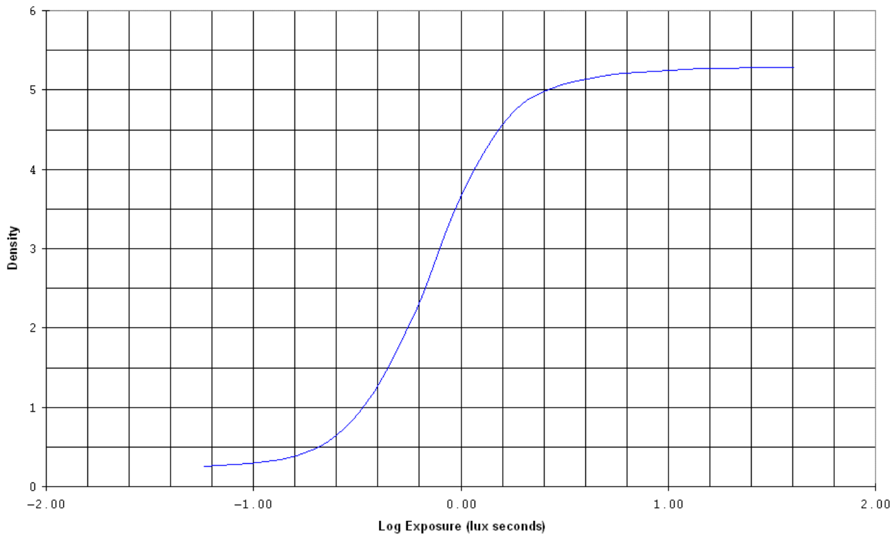
TI2292C 4-01 CHARACTERISTIC, For Publication KODAK Panchromatic Sound Recording Film 2374 Tungsten (2850K) plus KODAK Heat Absorbing Glass, No.2043,1/1000 sec. KODAK Developer D-97, 4 min, 75F (24C); Diffuse visual
