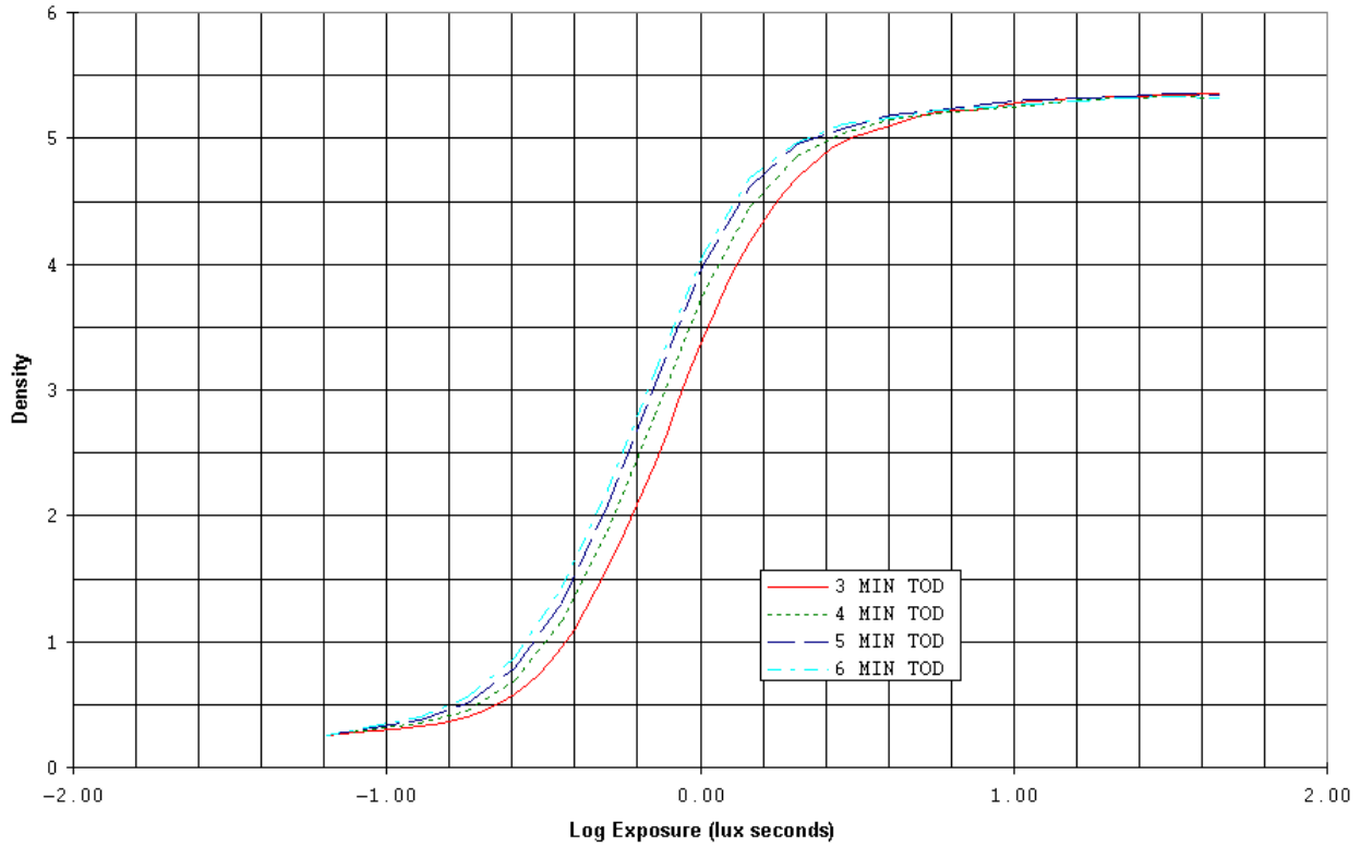
TI2292G 3-01 CHARACTERISTIC - TIME OF DEVELOPMENT, For Publication KODAK Panchromatic Sound Recording Film 2374 Tungsten (2850K) plus KODAK Heat Absorbing Glass, No.2043,1/1000 sec. Diffuse visual
